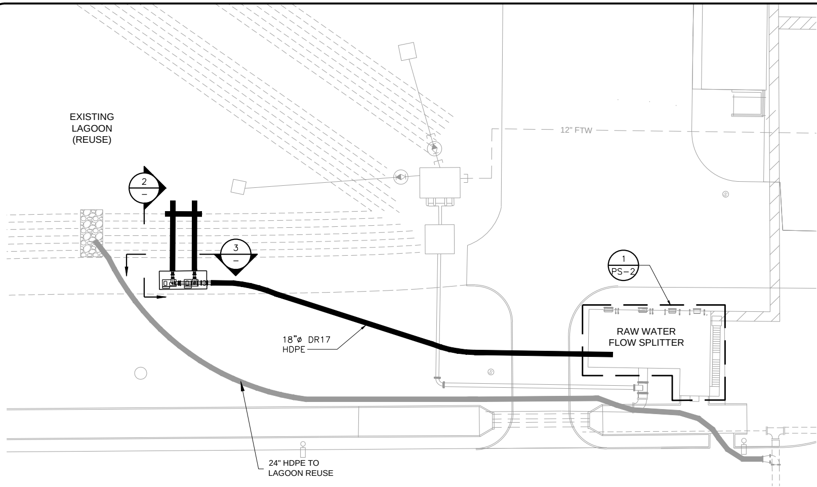
1 AREA PLAN 1"=20'
